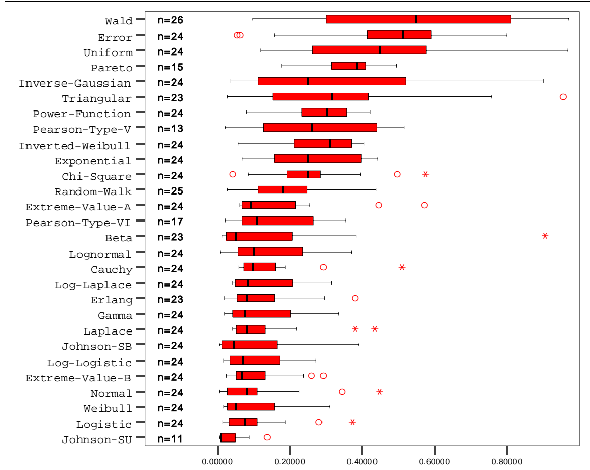
Figure 8 Maximum difference in density function, all experiments and all distributions
